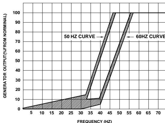
Figure 3 Frequency Compensation Curves
