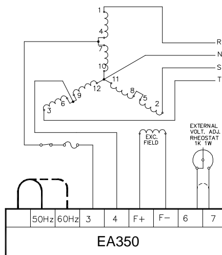
Figure 7 3Ø 380VAC Diagram
